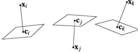
Figure 7.1: . An illustration of our surfel representation. Each data point x_i is associated with a piece of plane, which represents the surface of the underlying object. Surfel centers c_i are the projections of data points x_i to surfel planes.
