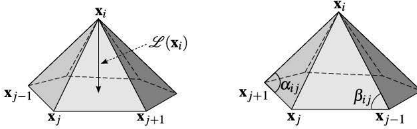
Figure 5.3: On the left an umbrella operator evaluated as a vector joining the vertex at position \mathbf{x}_i to the average of its neighbors. The origin of the name is obvious from the illustration. On the right the angles used for weighting the contribution of the edge e_{ij} to the mean curvature normal of the top vertex.
