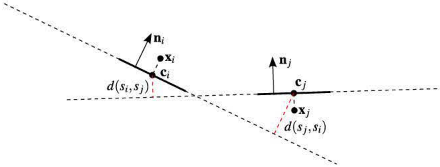
Figure 7.2: An illustration of the overlap potential, but in 2D. For the two neighboring surfels s_i and s_j we consider the projection of the center c_i to the plane of s_j , and vice versa. The lengths of those projections (marked in red) are the terms we want to minimize in order to achieve the best overlap.
