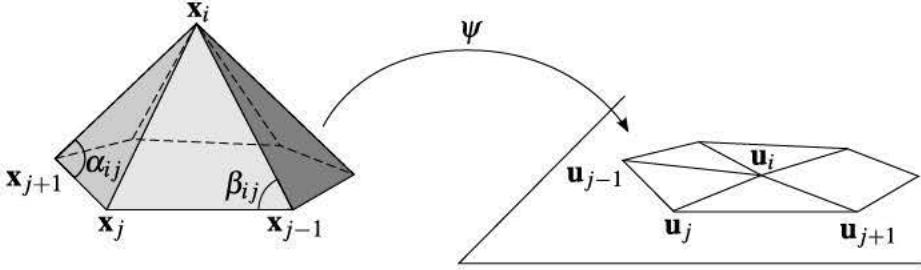
Figure 5.11: A 3D 1-ring of the original mesh and its associated flattened version in the parametrization domain.
