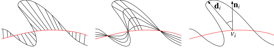
Figure 8.4: Left: geometric texture superimposed on objects's base shape in form of vector displacements. The points at the intersections of the textured surface and the base shape have zero displacements. Middle: One way of obtaining the base shape in case of non-heightfield texture would be to use the multiresolution hierarchies as in [79] and trace the points through a sufficient number of levels. Right: The displacement \mathbf{d} of the vertex v_i can be described in terms of displacement length and the rotation from the normal vector.
