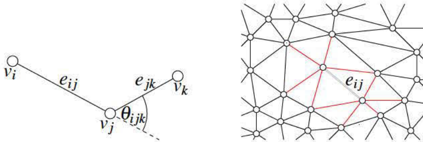
Figure 6.2: Left : A pair of edges. The support for the edges e_{ij} and e_{jk} depends on the size of the angle \theta_{ijk} . Right : A neighborhood structure for the edge support. The neighbors of the edge e_{ij} are marked red. Neighboring edges support each other if they lie along the same line.
