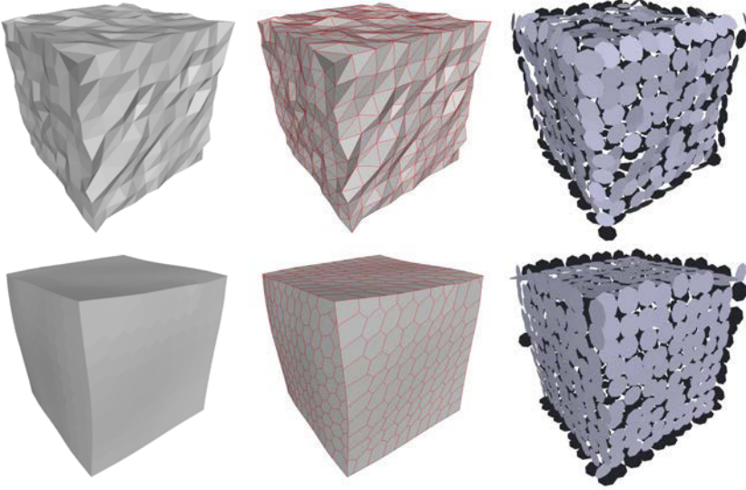
Figure 7.4: The reconstruction of a synthetic cube corrupted by Gaussian noise. Top : Two renderings of the input mesh and the initial surfel configuration. Bottom : Corresponding renderings of the reconstructed surface and optimized surfel configuration. Parameters used: data weight \alpha = 0.01 , parallelism weight \beta = 100 , angle threshold t set to exponentially decrease between 45^\circ and 10^\circ . The result was obtained in 10 iterations.
