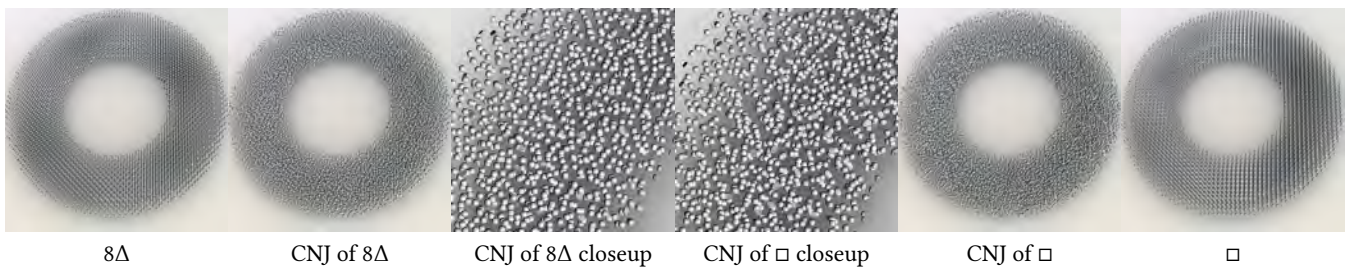
Figure 10: To indicate the difference between the cubic grid ( \square ) and the octahedral grid ( 8\Delta ), we here show the point distributions for the copper foam scene when using the two different types of initial grid. We tried to obtain a similar result with both grids. Due to the larger distance between the nodes in the cubic grid, we made the grid smaller, applied a larger time step, and decreased the scale in CNJ. The distribution of points is more uneven for the cubic grid.
