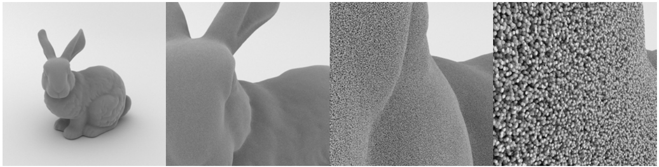
Figure 8: Moving closer and closer to a seemingly dusty version of the Stanford bunny ( http://graphics.stanford.edu/data/3D-scanrep/ ). This illustrates our ability to distribute a very large number of points using CNJ w. SoS and RK4. Rendering time for a 1spp frame (left to right): 2.5 s, 4.5 s, 5.4 s, 6.4 s. Rendered here with 3000 samples per pixel.
