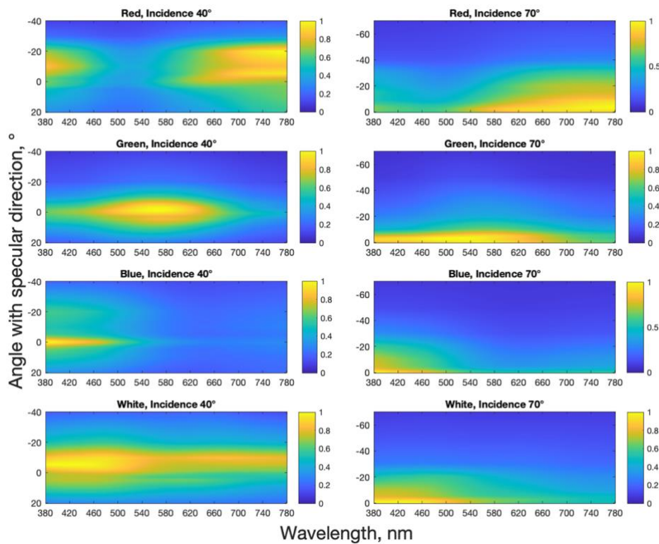
Figure 3 Scaled reflected spectra for angles of incidence ( 40^\circ and 70^\circ ) for reflected angles with respect to the specular reflection direction. Spectra of samples with 30% pigment concentration and 4 applied layers are demonstrated.
