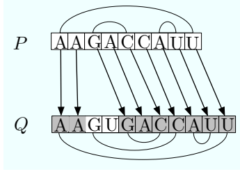
Figure 2: An embedding of P in Q . f(1) = 1, f(2) = 2 and f(j) = j + 2 for j = 3, 4, \dots, 9 . A_P = \{(1, 9), (3, 5), (7, 8)\} and A_Q = \{(1, 11), (3, 8), (5, 7), (9, 10)\} . We have (f(1), f(9)) = (1, 11) \in A_Q , (f(3), f(5)) = (5, 7) \in A_Q , and (f(7), f(8)) = (9, 10) \in A_Q .
