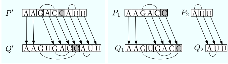
Figure 3: Illustration of the Splitting Lemma. Index i = 8 induces an arc-preserving split of Q' with Q_1 = Q'[1, 8] and Q_2 = Q'[9, 11] . Index j = 6 induces an arc-preserving split of P' with P_1 = P'[1, 6] and P_2 = P'[7, 9] such that P_1 \sqsubseteq Q_1 and P_2 \sqsubseteq Q_2 .
