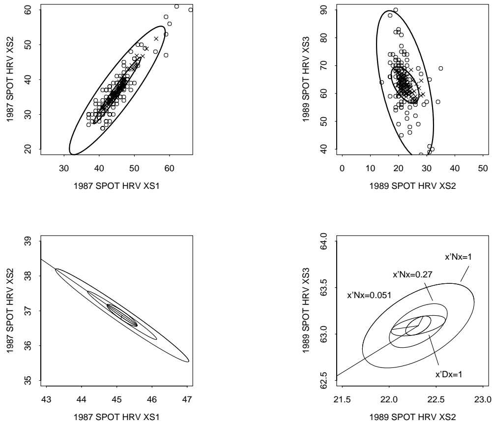
Figure 5: Canonical variates geometrically
