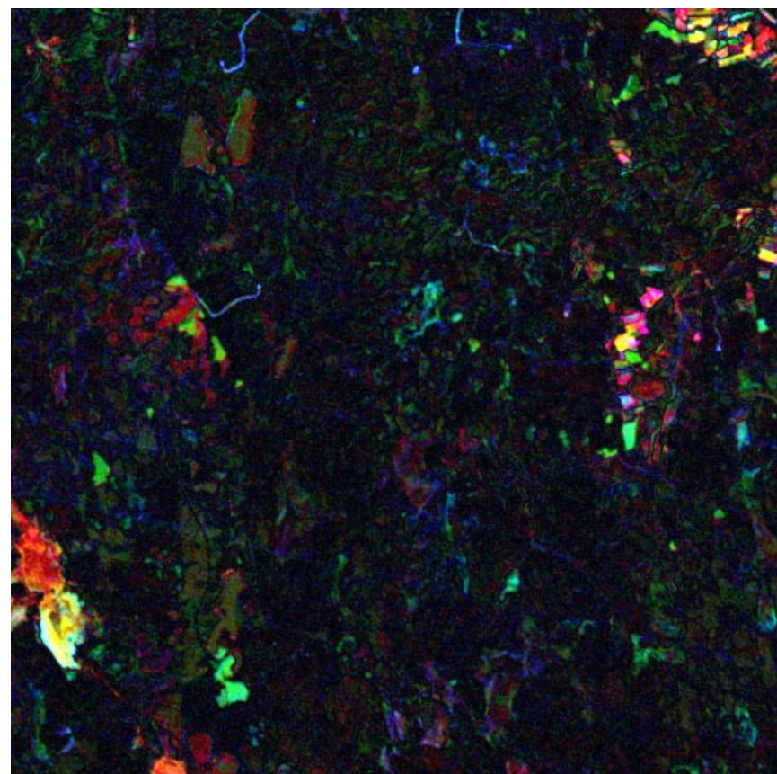
Figure 3.36: Absolute values of MAFs 1, 2 and 3 of MADs of TM bands from 1986 and 1988 as RGB
