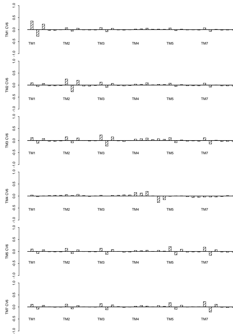
Figure 3.28: Correlations between Q-mode CVs 6 and original data
