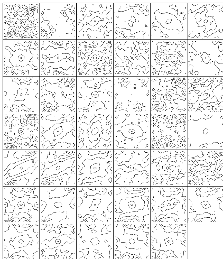
Figure 1.11: 2-D semivariograms for 41 geochemical elements in South Greenland, 21 \times 21 5 km pixels as contour plots
