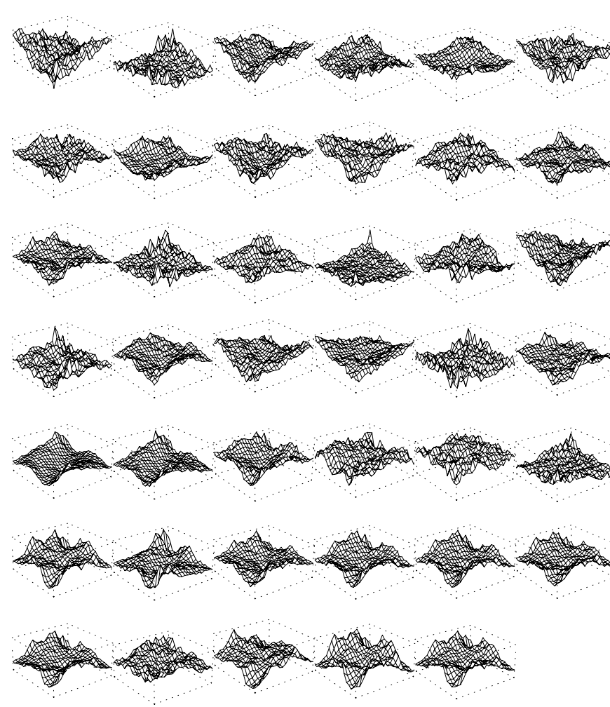
Figure 1.12: 2-D semivariograms for 41 geochemical elements in South Greenland, 21 \times 21 5 km pixels as perspective plots
